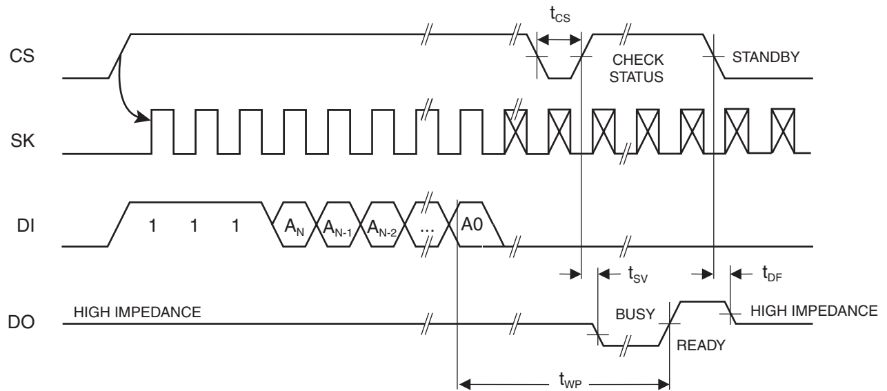
Figure 8. ERASE Timing
