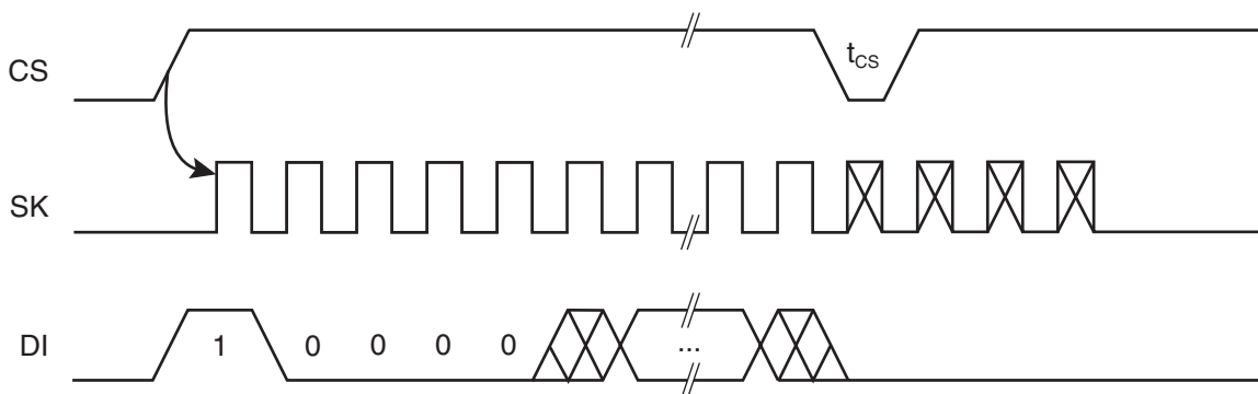
Figure 5. EWDS Timing
