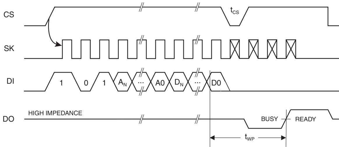
Figure 6. WRITE Timing
