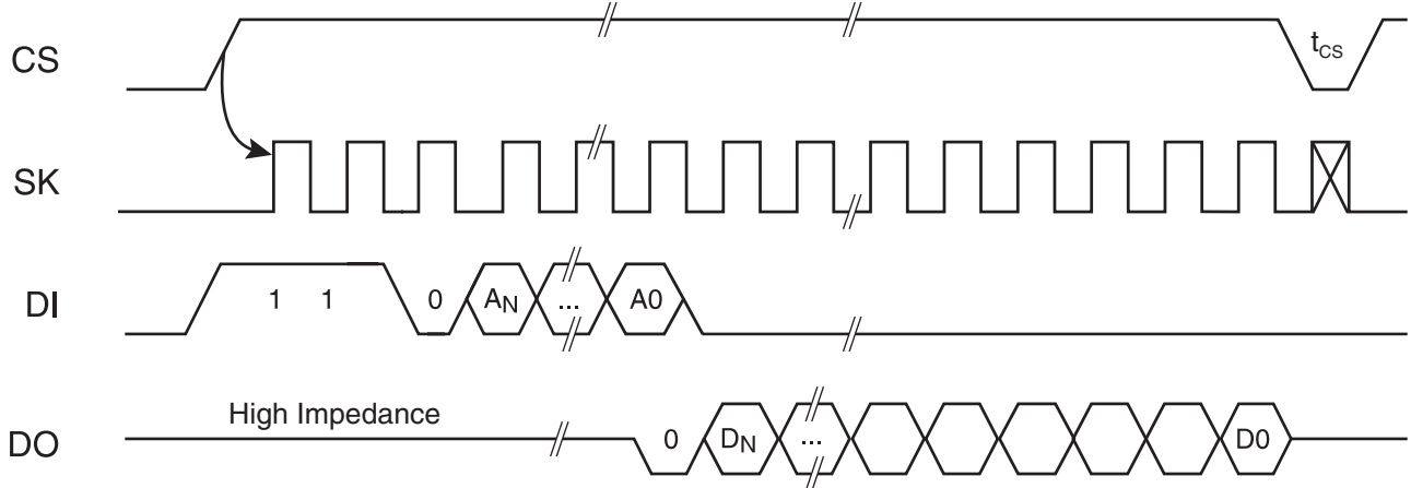
Figure 3. READ Timing
