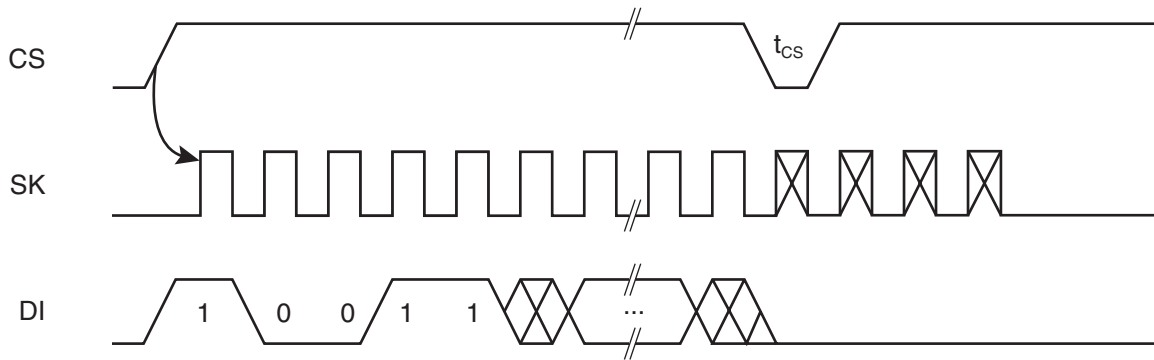
Figure 4. EWEN Timing
