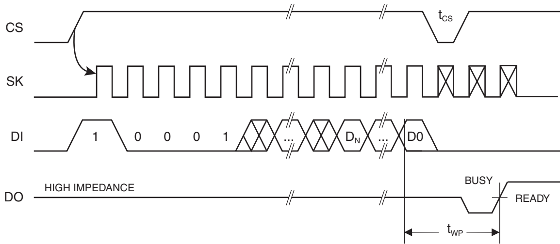
Figure 7. WRAL Timing (1)
